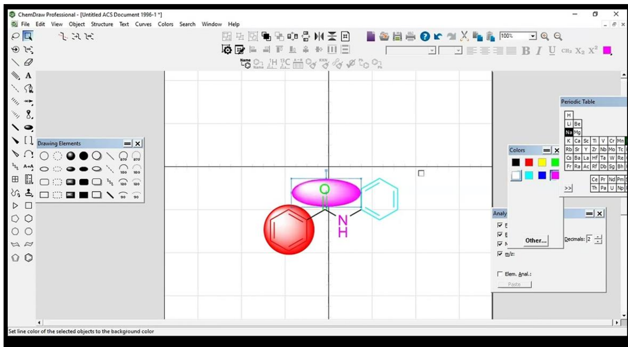
Screenshot of ChemDraw ultra 12 software structure drawing images.
