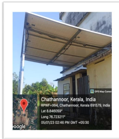
1.5 KW x 3 KV solar off grid power system installed at SN College Chathannur.
